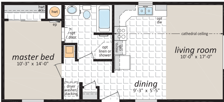
CJS-1821, 18' x 40' - 720 sq. ft.
