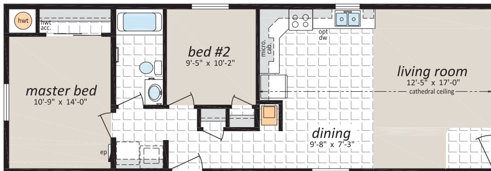
CJS-1827, 18' x 60' - 1,080 sq. ft.
