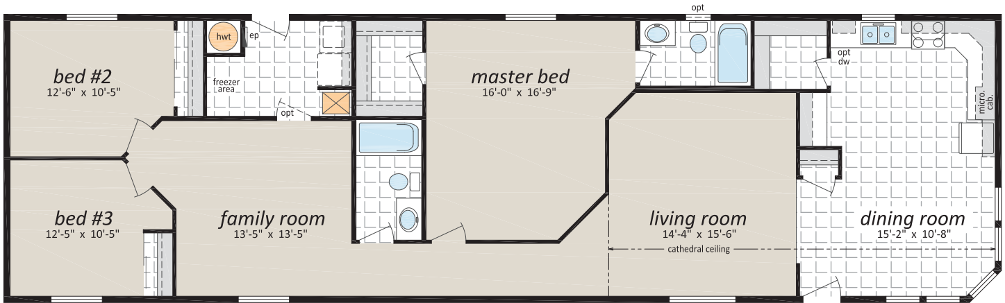
CJS-2214, 22' x 76' - 1,672 sq. ft.
