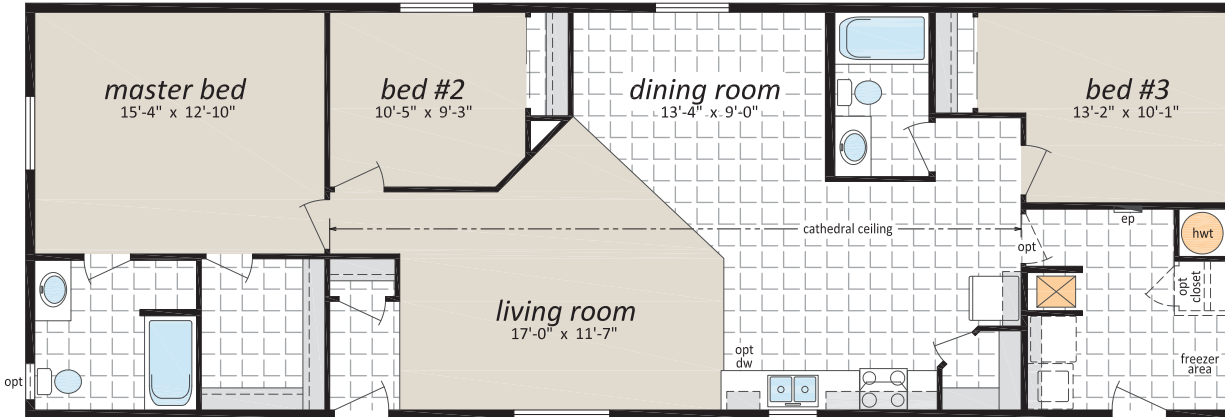
CJS-2206, 22' x 64' - 1,408 sq. ft.
