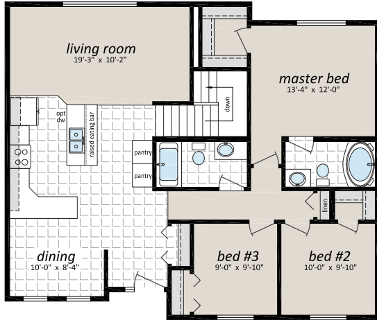
ACC 3440, "The Manchester" 34' x 40', 1,290 Sq. Ft. 3 Bedrooms, 2 Baths Shown with Optional Exterior Features
