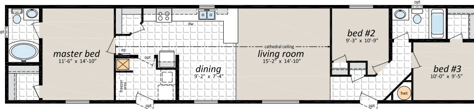
SWII-20, 16' x 76', 1,216 Sq. Ft., 3 Bedrooms, 2 Baths
