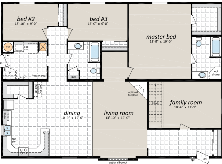
CJS-4056, 40'x 56', 2,240 Sq. Ft., 3 Bedrooms, 2 Baths
