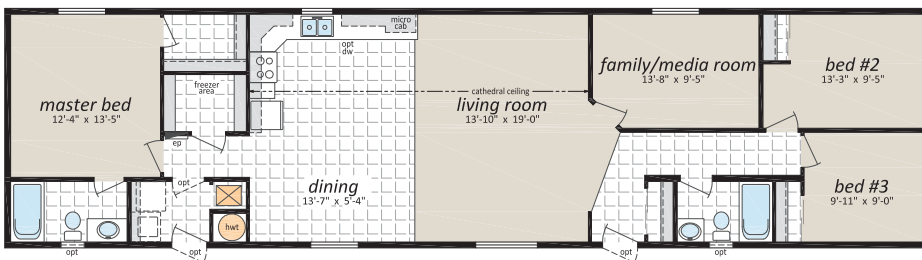
CJS-3011, 20'x 76', 1,520 Sq. Ft., 3 Bedrooms, 2 Baths, FR
