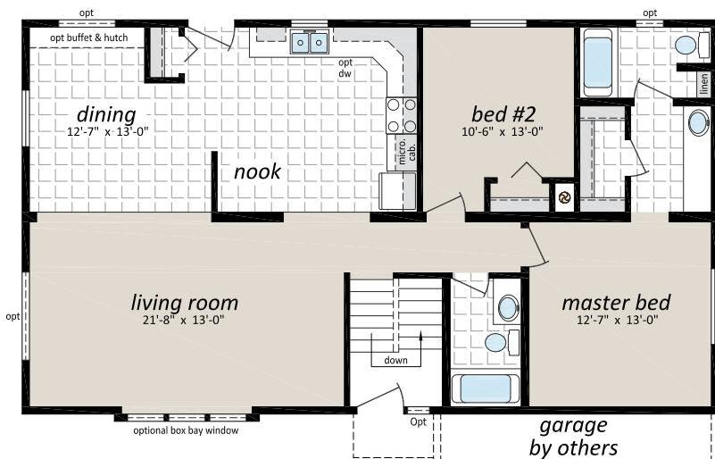
SSM-816F, "The Webster" 27'6" x 48', 1,320 Sq. Ft., 2 Bedrooms, 2 Baths
