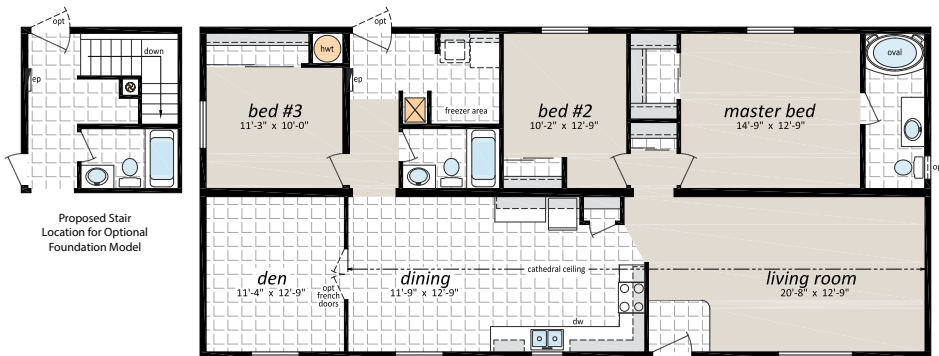
SWII-314, 27'-6" x 60', 1,650 Sq. Ft., 3 Bedrooms, 2 Baths
