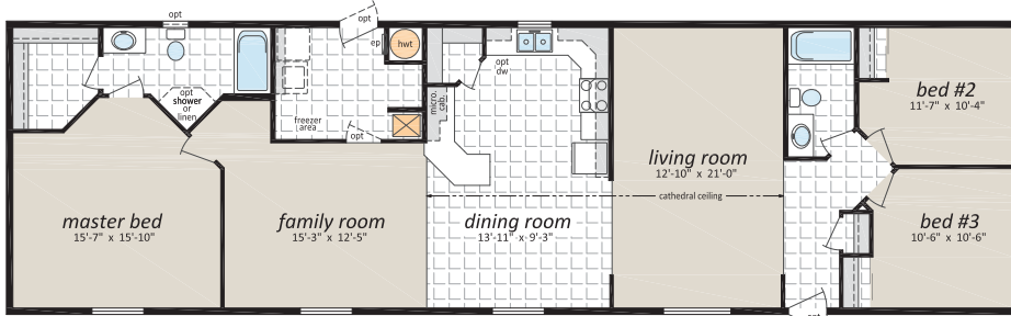
CJS-2212, 22'x 76', 1,672 Sq. Ft., 3 Bedrooms, 2 Baths, FR
