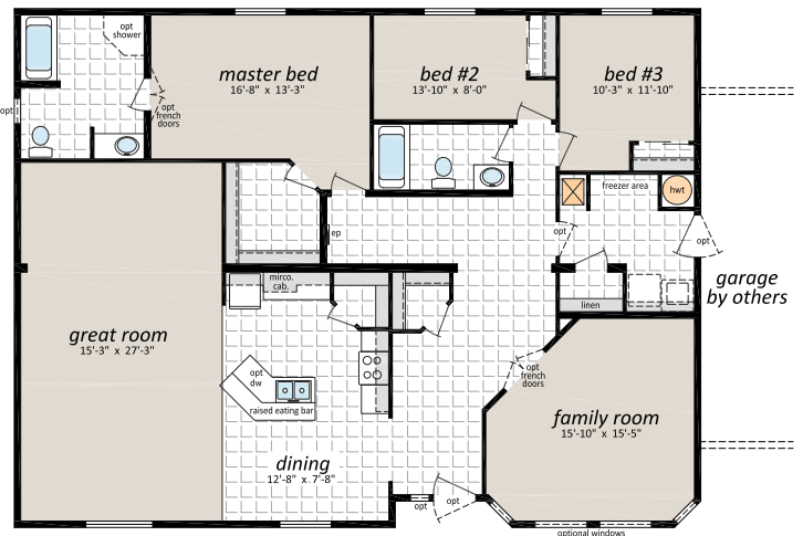
CJS-4052, 40'x 52', 2,080 Sq. Ft., 3 Bedrooms, 2 Baths
