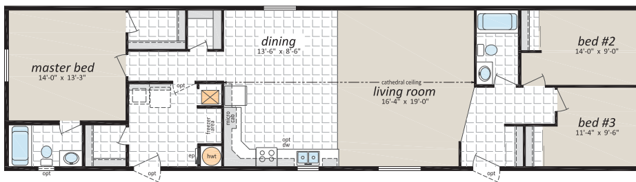
CJS-3022, 20'x 76', 1,520 Sq. Ft., 3 Bedrooms, 2 Baths
