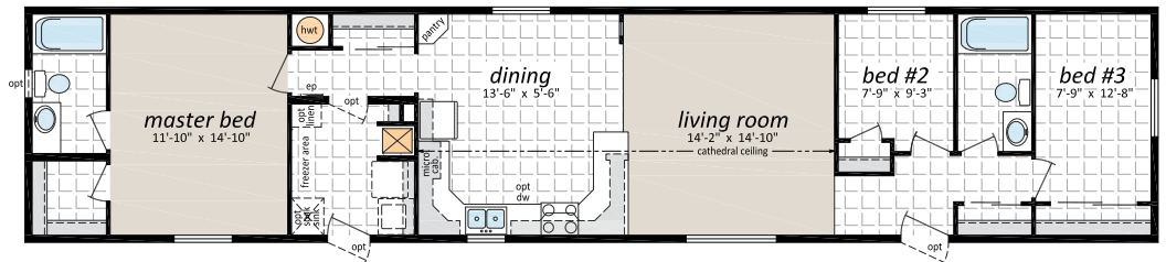
SP-1005A, 16'x 76', 1,216 Sq. Ft., 3 Bedrooms, 2 Baths
