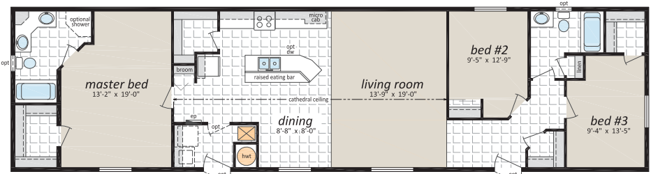
CJS-3019, 20' x 76', 1,520 Sq. Ft., 3 Bedrooms, 2 Baths
