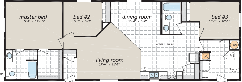
CJS-2206, 22'x 64', 1,408 Sq. Ft., 3 Bedrooms, 2 Baths
