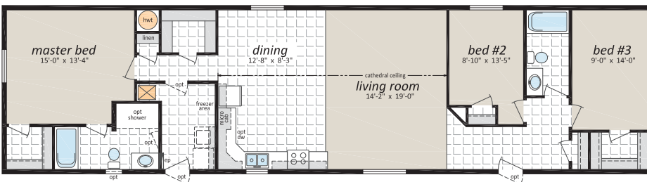
CJS-3022, 20'x 76', 1,520 Sq. Ft., 3 Bedrooms, 2 Baths
