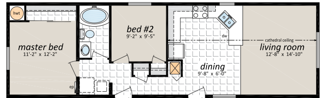
SWII-08, 16' x 52', 832 Sq. Ft., 2 Bedrooms, 1 Bath
