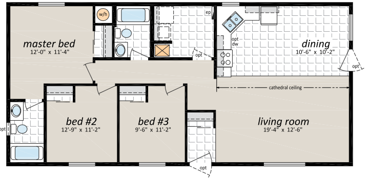
RTM-24003, 24' x 50', 1,200 Sq. Ft. 3 Bedrooms, 2 Baths
