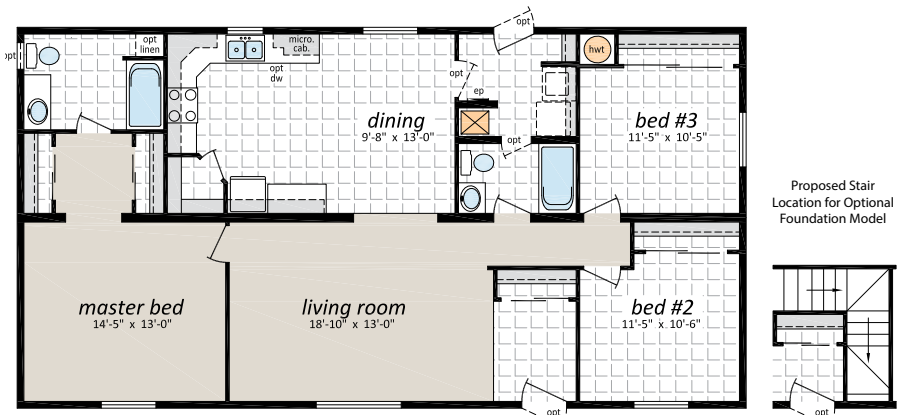
SP-1204, 27'6" x 52', 1,430 Sq. Ft., 3 Bedrooms, 2 Baths
