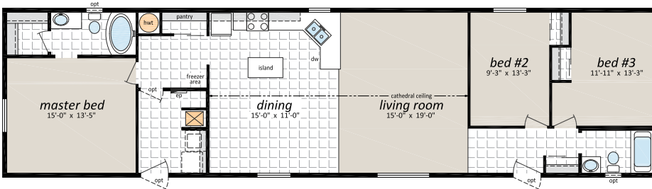
SWII-224, 20' x 76', 1,520 Sq. Ft., 3 Bedrooms, 2 Baths
