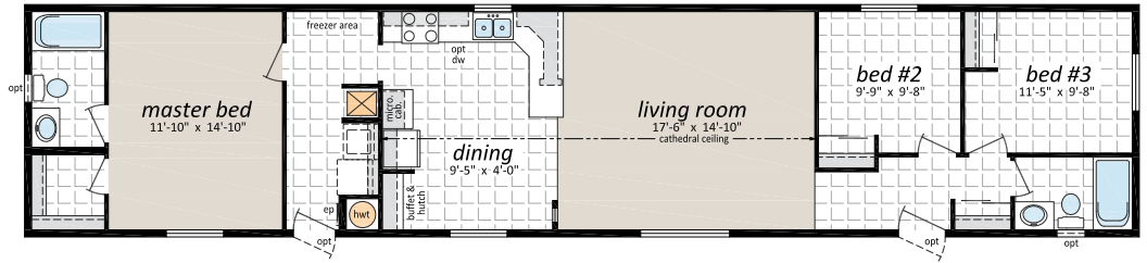
SP-1000A, 16'x 76', 1,216 Sq. Ft., 3 Bedrooms, 2 Baths
