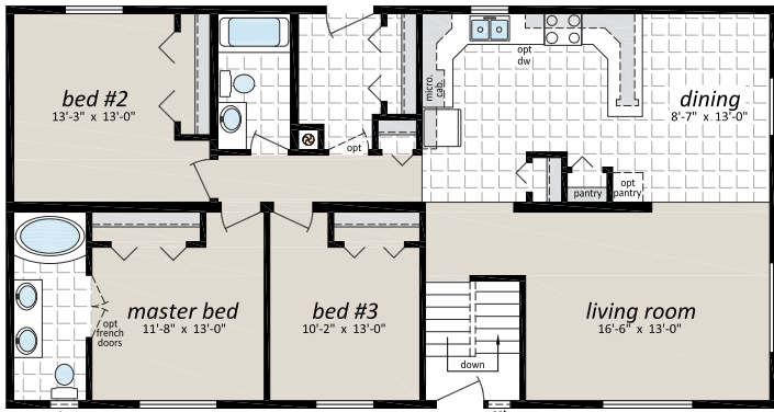
SSM-802F, "The Lancaster" 27'6" x 52', 1,430 Sq. Ft., 3 Bedrooms, 2 Baths Shown with Optional Exterior Features
